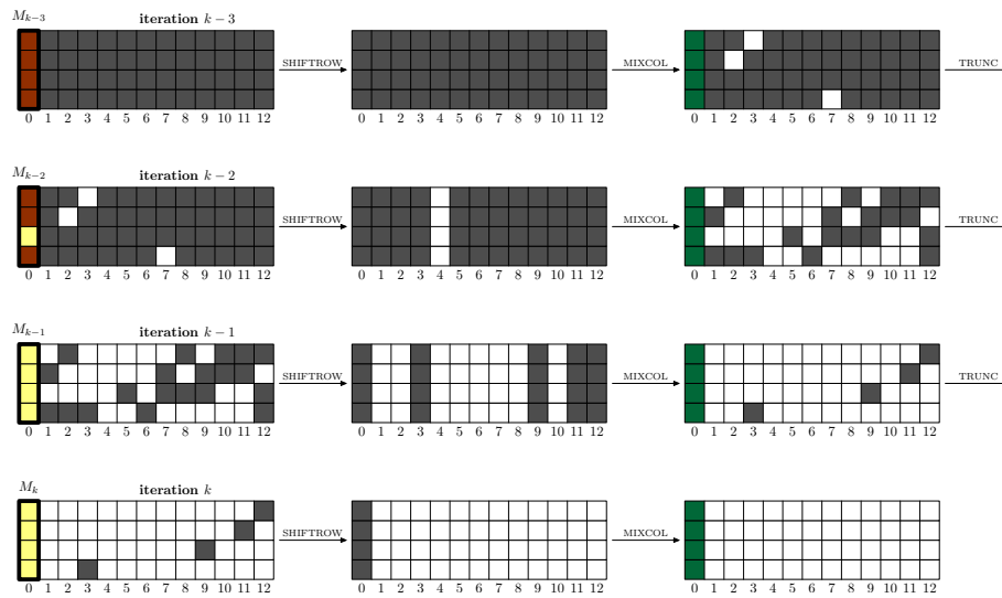
Fig. 2. Truncated-differential path in 4 iterations starting from an all-difference pair of states, to be used for a second preimage attack.
